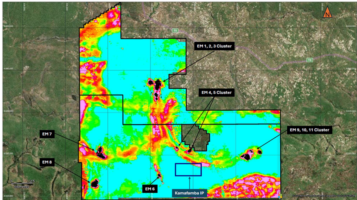
Figure 9: Mumbenzi Project – Licence wide processed EM geophysical output showing Tau Decay Constant data
