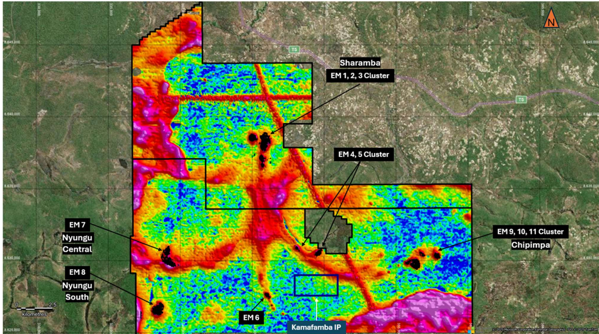
Figure 8: Mumbenzi Project – Licence wide processed EM geophysical output showing identified strong EM conductors and prospect locations
