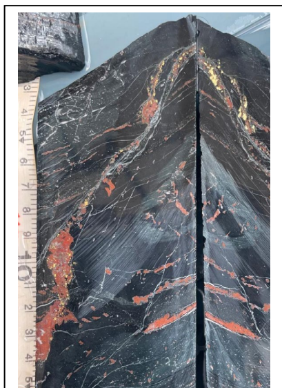
Plate 1 - SDH25-028, 305.5 meters down Hole, Visible gold in cut core, He Mt hosted. Assay reported.
