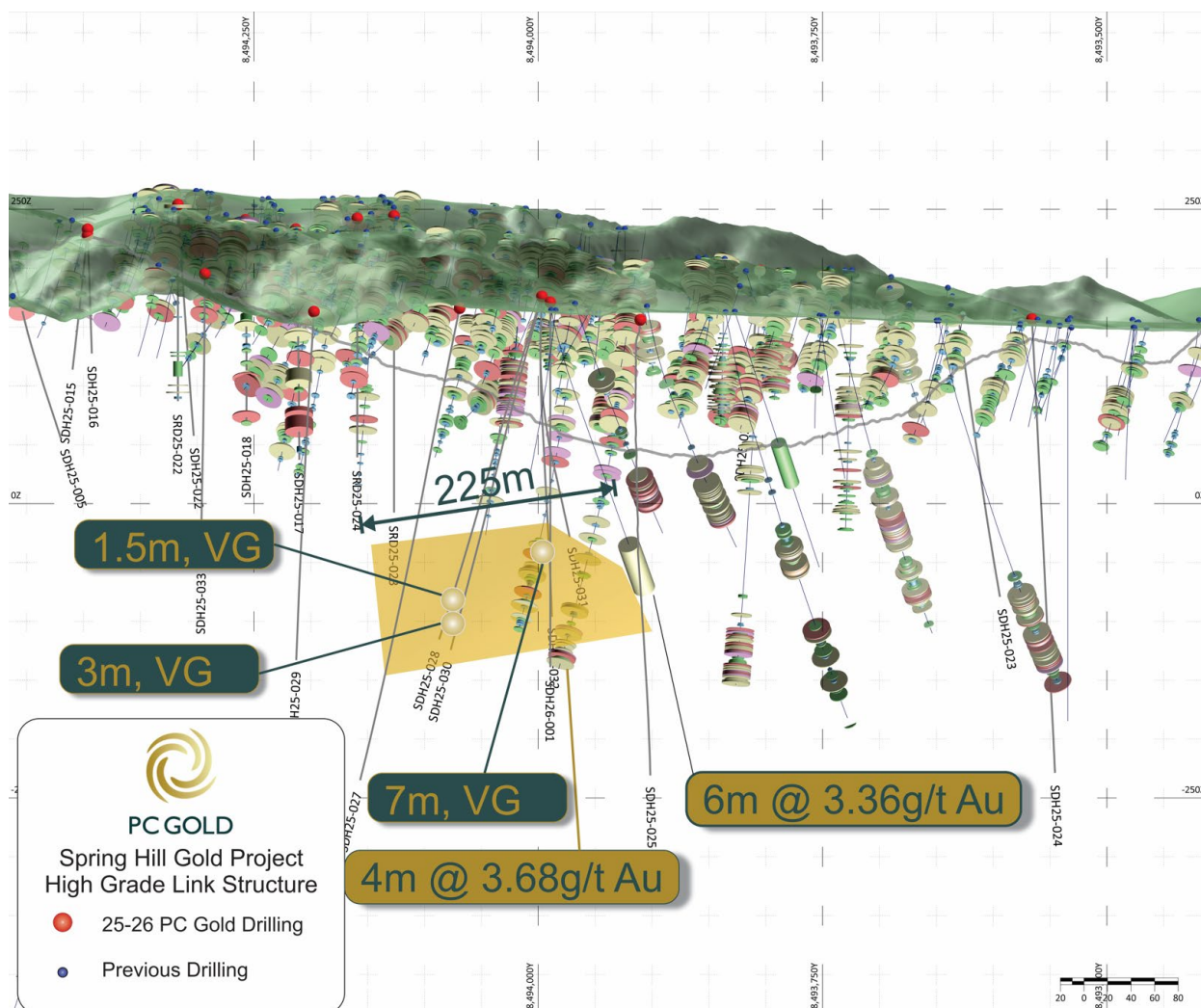
Figure 3 - High-grade link structure between HK and Macap with the current Pit shell and current and past drilling
