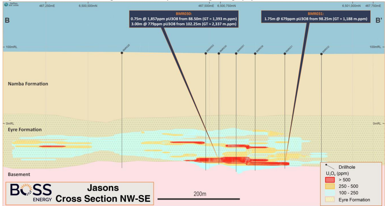
Figure 7: Cross section A-A through the Jason's Deposit showing stratigraphy and the MRE block model.
