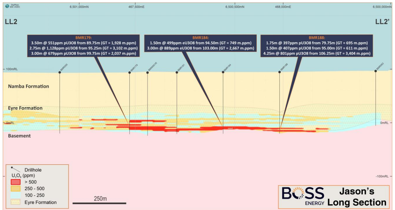
Figure 8: Long section through the Jason's Deposit showing the multiple mineralised horizons. The main horizon is the basal sequence.
